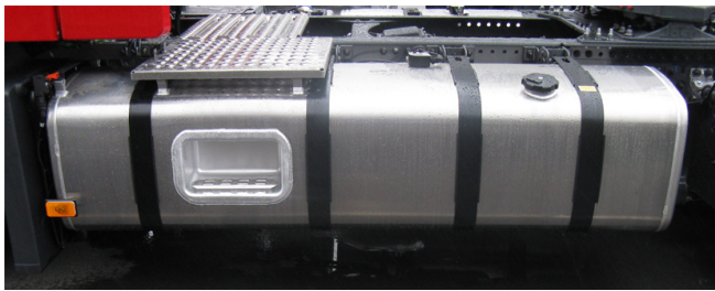
Left hand mounted fuel tank in aluminium with steps – D56.
