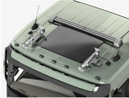
FH Sleeper Cab, HORN-R2S, ACCBR-M.
