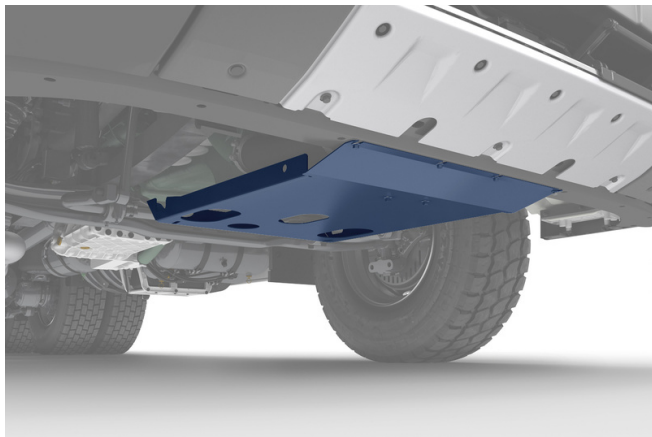
GUARD-EH, non driving front axle.
