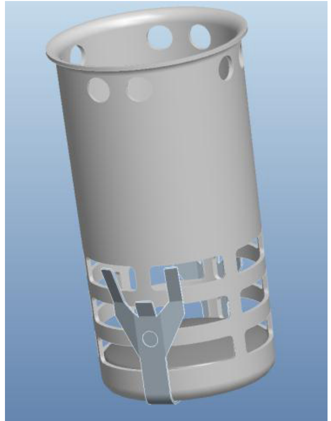
FUFF-ATS with anti-theft and anti-spillage function.
