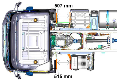
Free Frame Space with one front axle and day cab.
