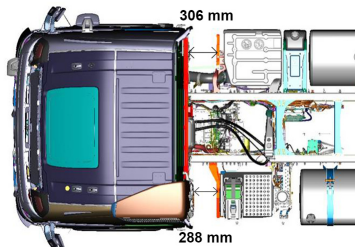
Free Frame Space with one front axle and all sleeper cabs.
