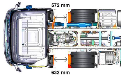
Free Frame Space with two front axles and day cab.
