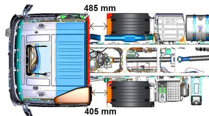
Free Frame Space with two front axles and all sleeper cabs.
