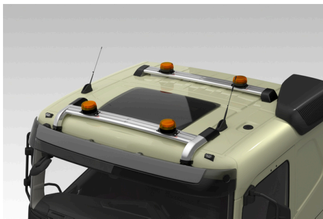
Volvo FMX Sleeper Cab with BEACONA4, ACCRB-F and ACCRB-R.
