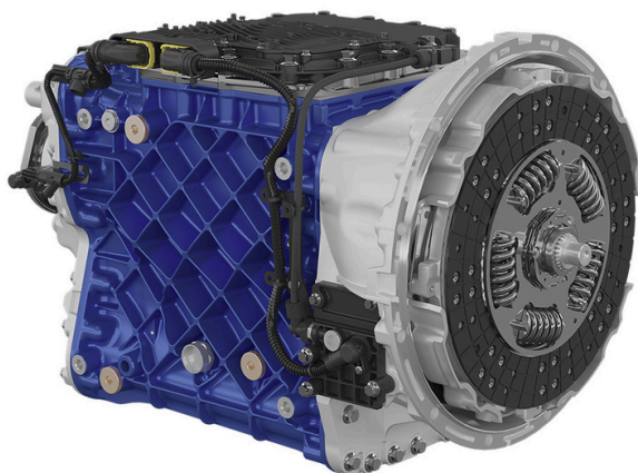
I-Shift – 12-speed – automated gearbox.
