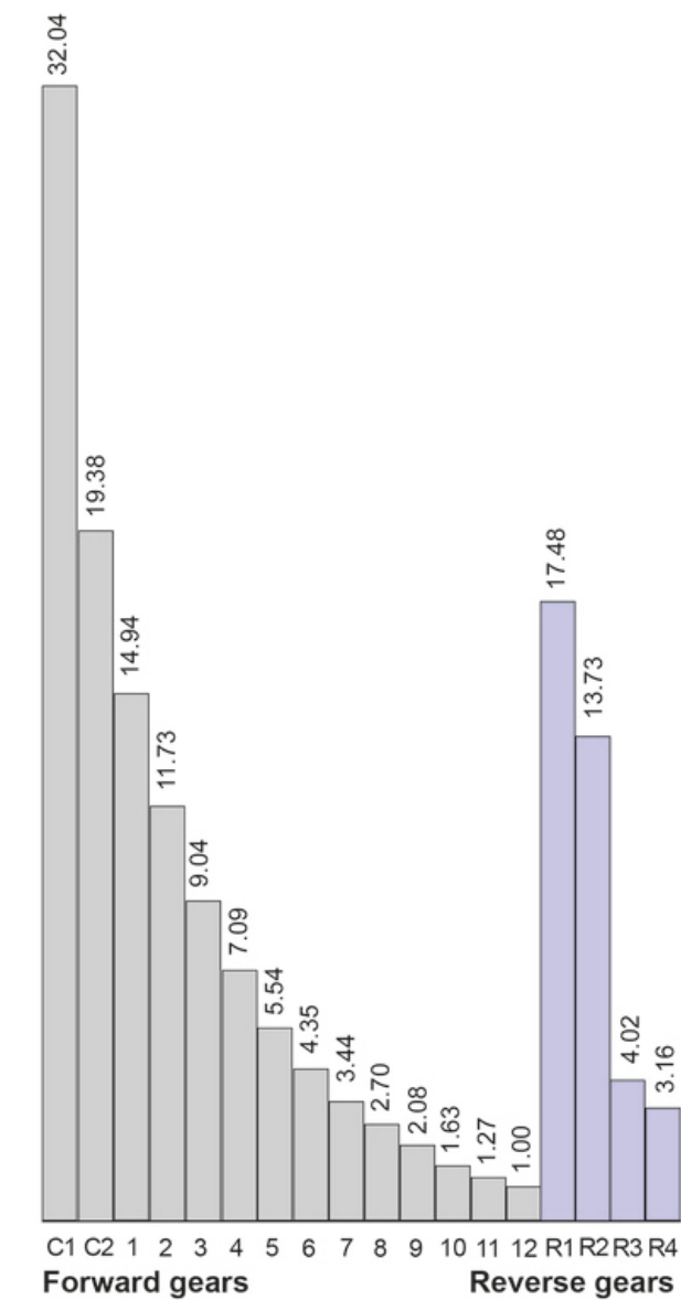
Ratios AT2612 with ASO-ULC
