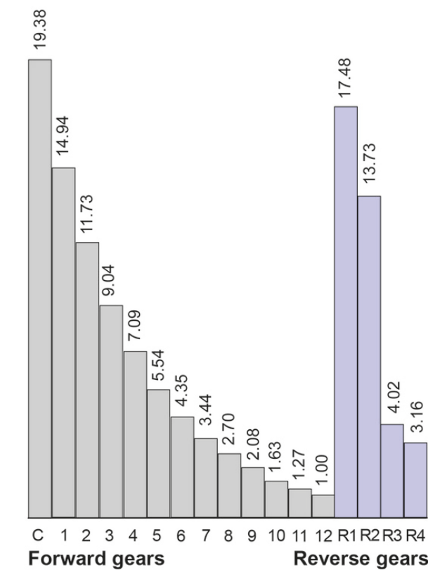
Ratios AT2612 with ASO-C
