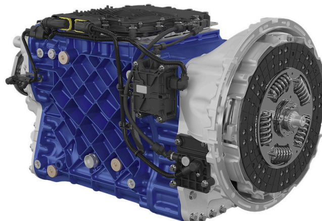
I-Shift with crawler gears. It has an extension unit between the clutch and the gearbox - enabling 13 or 14 gear with possibility of additional reverse gears. Includes options ASO-C/ASO-ULC/ARSO-MSR.
