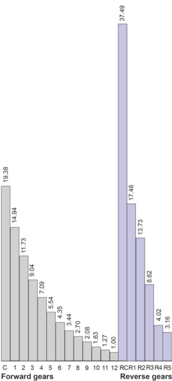
Ratios AT2612 with ASO-C and ARSO-MSR
